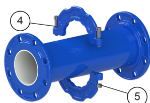
Adjustable puddle flanged DN 50 up to DN 200
