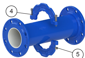
Ajustable puddle flanged DN 50 up to DN 200
