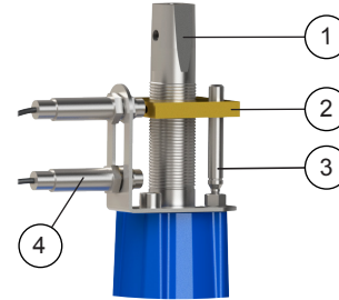
Position indicator & open-close limit switch detail
