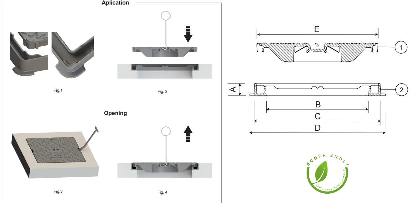
Fig.1 - Anti-noise locking system
