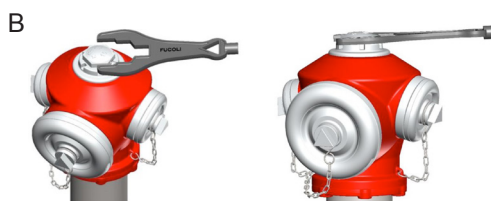
Opening and closing operation of the Ignis fire hydrant [ref. 07.700]
